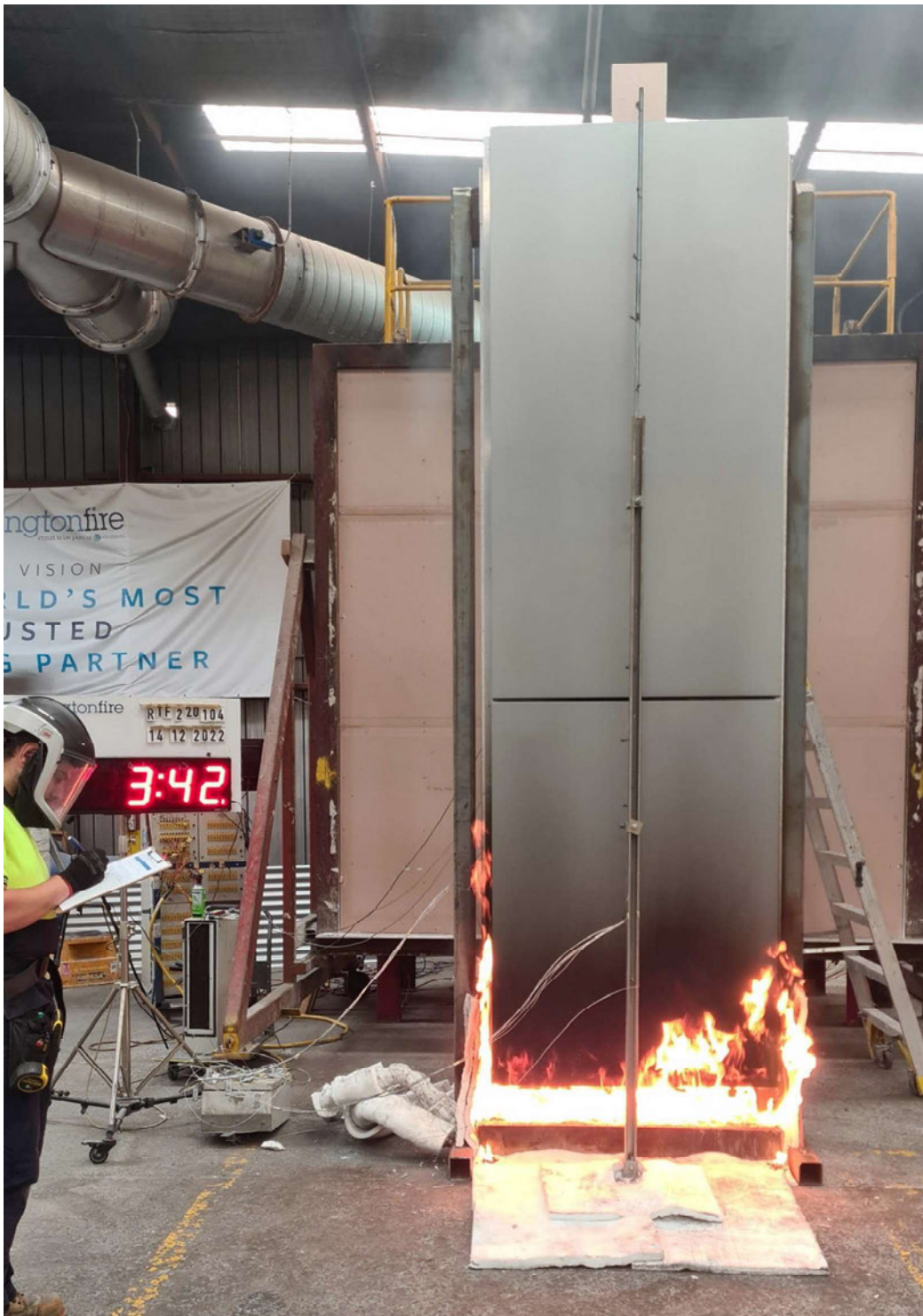
Figure 10 The specimen 3 minutes 42 seconds into the test (burner output at 100 kW)
