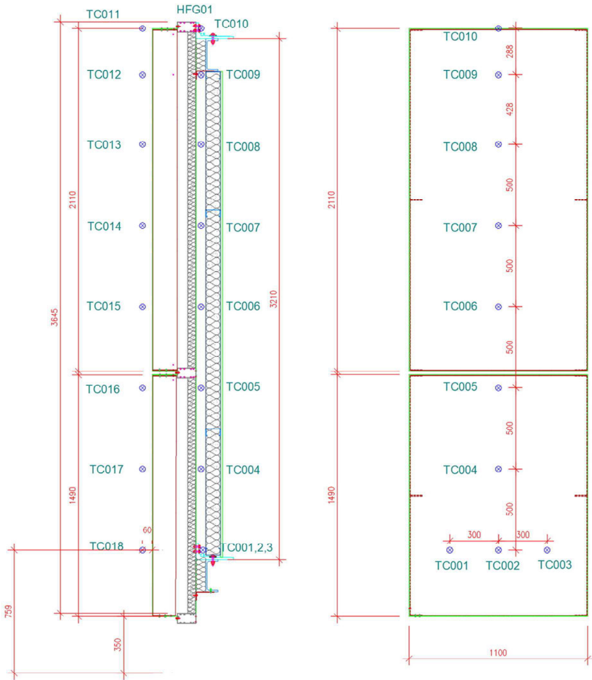
Figure 1 Instrumentation location
