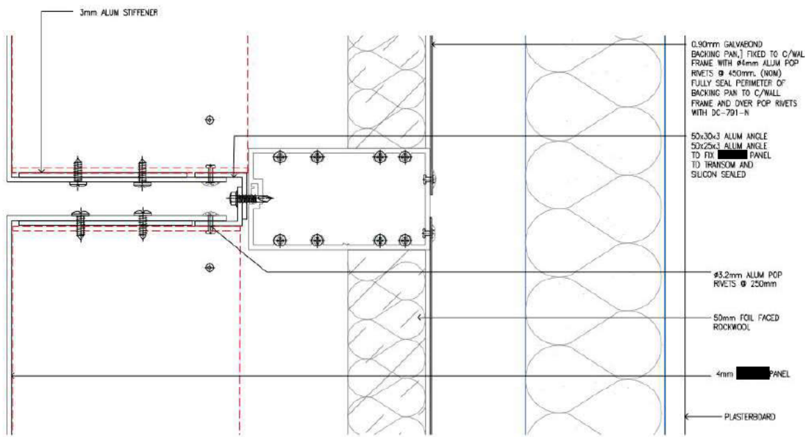
Figure 8 System assembly – middle join detail (D05)
