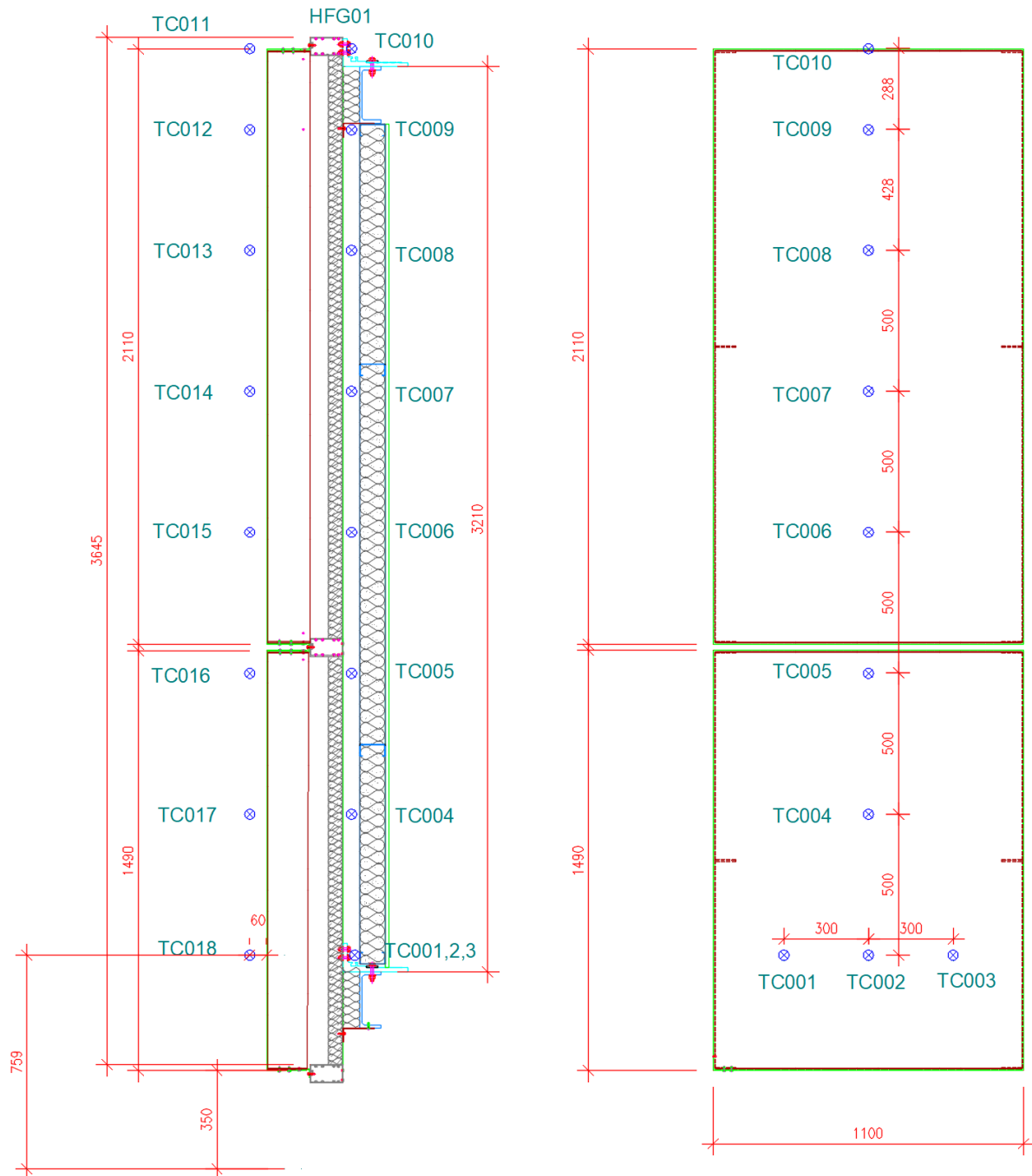
Figure 1 Instrumentation location
