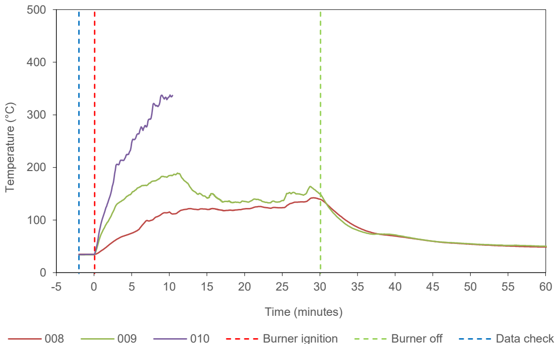
Figure 4 External temperature data collected by plate thermocouples in-line with ACP, above and below, respectively - in-line with the burner 1
