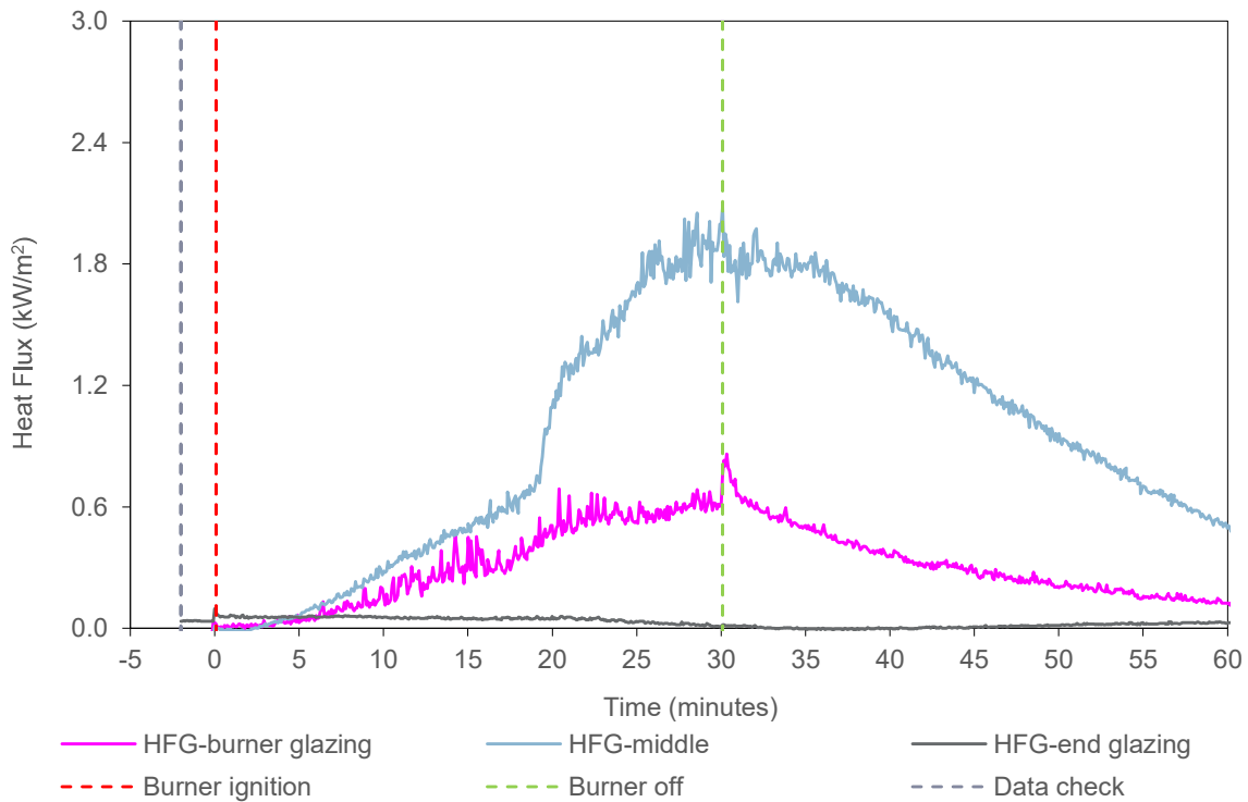
Figure 10 Heat flux data collected by heat flux gauges behind the glazing units
